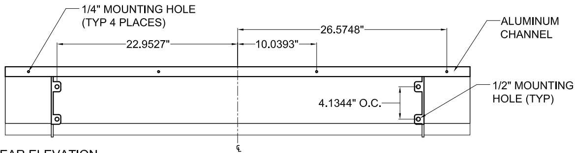
REAR ELEVATION
