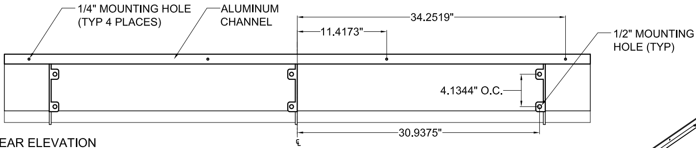
REAR ELEVATION
