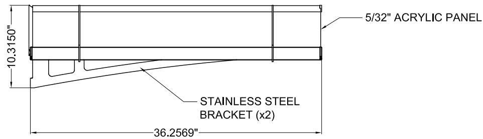
PROFILE ELEVATION
