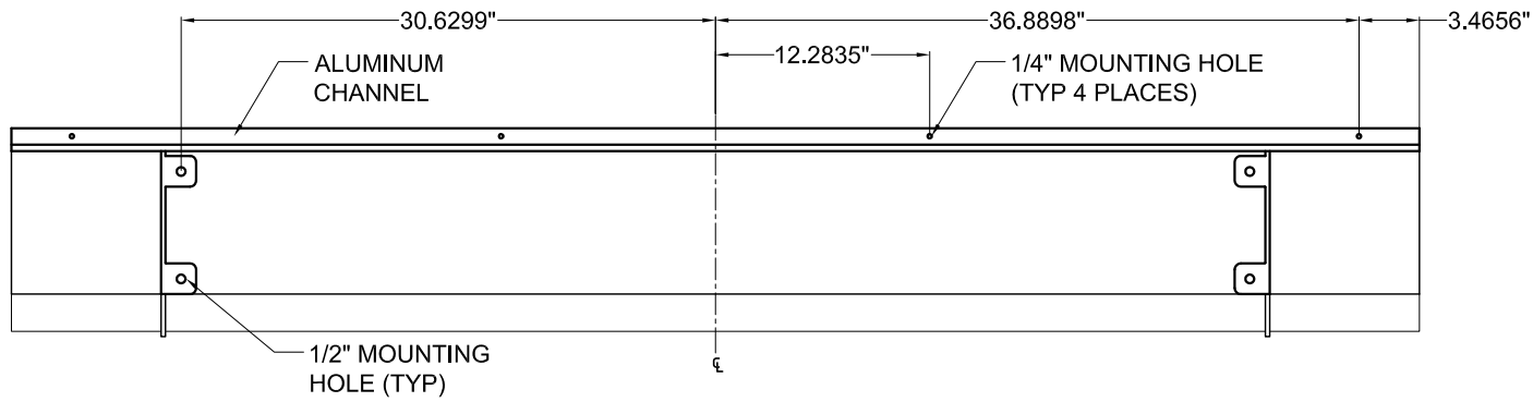
REAR ELEVATION
